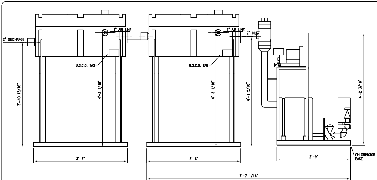
ASSEMBLY
