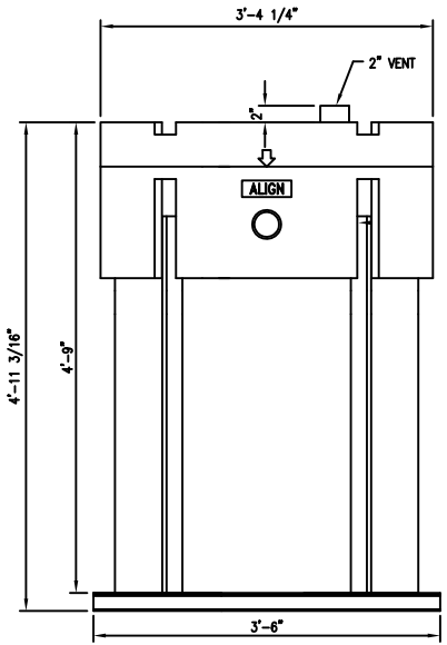
DISCHARGE VIEW
